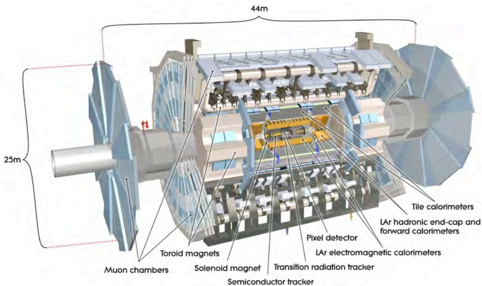
Figure 28.5: Cutaway view of the ATLAS detector. The detector is 25m in height and 44m in length (note the two persons as an indication of size). The overall weight of the detector is approximately 7000 tonnes. (CERN-GE-0803012 05 ©CERN)
