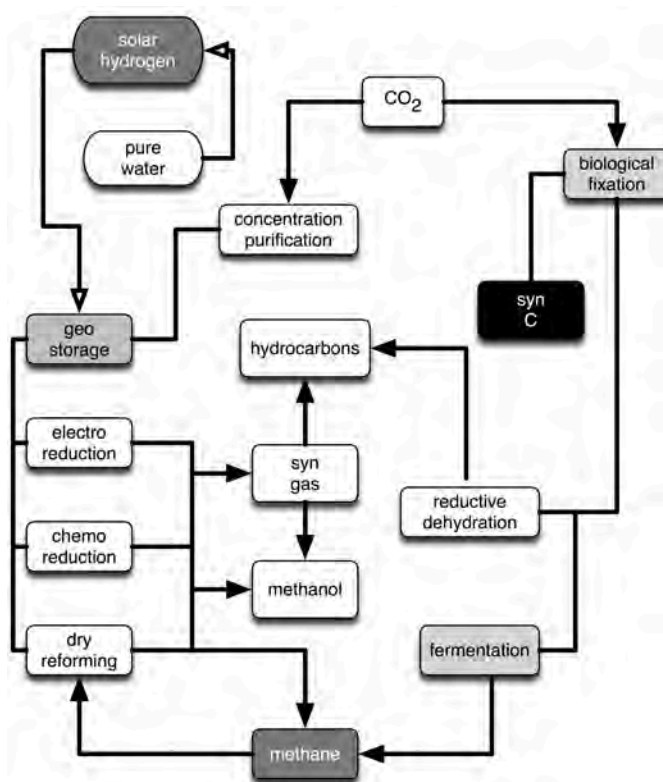
Figure 30.3: Uses of CO 2 as a raw material. Solar hydrogen is required in all conversion processes, including biological fixation. The boxes marked 'electro reduction,' 'chemo reduction,' 'dry reforming,' 'syn gas' and 'reductive dehydration' denote catalytic processes, the boxes 'fermentation' and 'biological fixation' stand for biological transformations. Methane is an intermediate product and energy carrier; the boxes 'hydrocarbons' and 'methanol' denote products for the chemical industry.
